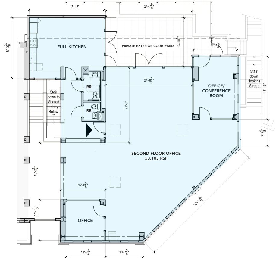
SECOND FLOOR
