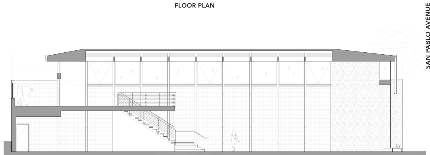
SECTION
